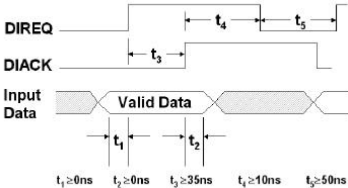
DIREQ & DIACK Handshaking
