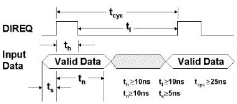
DIREQ as input data strobe (when Rising Edge Active)
