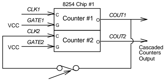
Figure 2.7 Example of 'user programmable cascaded counters'
